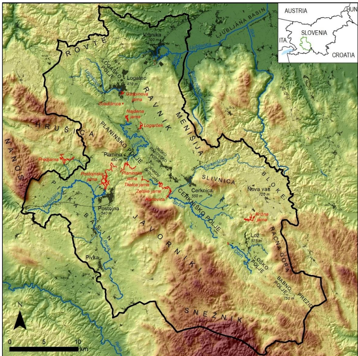
Figure 7: Map of the Ljubljana River recharge area covering most of the Notranjska Region, with high karstic plateaus, karst poljes and surface rivers. The main caves are shown with red lines.
